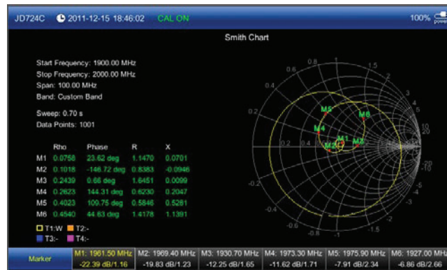
Smith Chart
